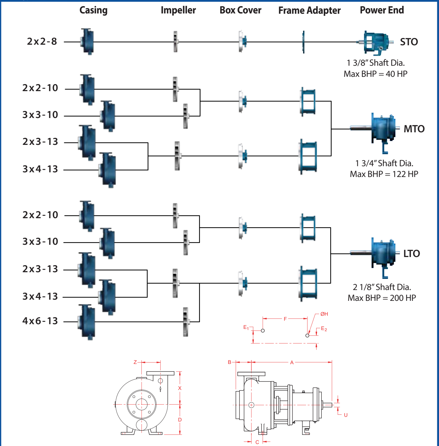
Pump Dimensions
