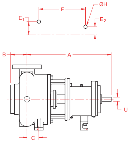
Pump Dimensions
